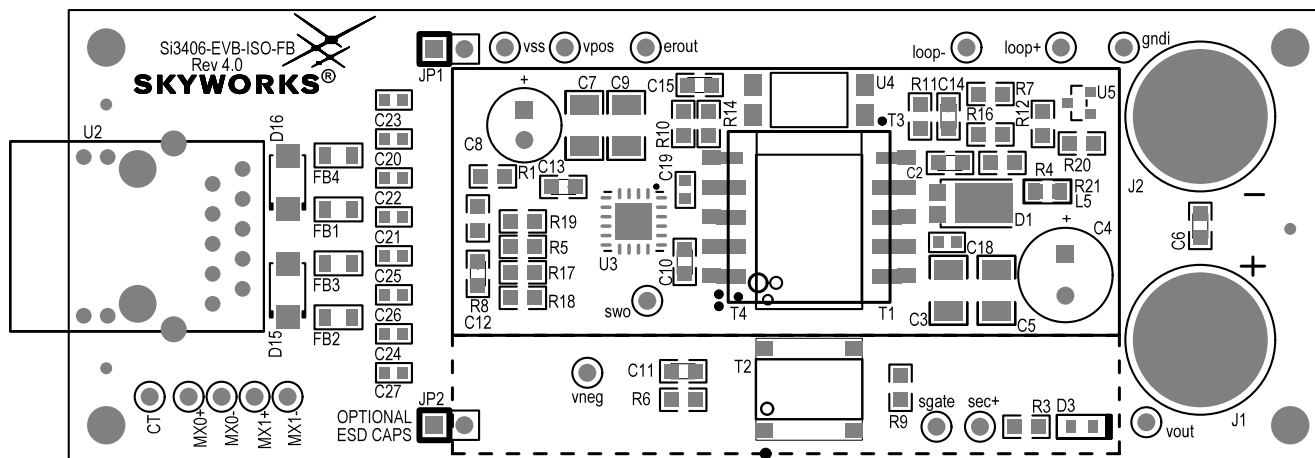
Figure 63. Top Silkscreen
