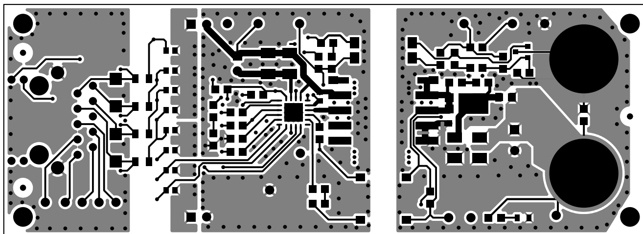
Figure 64. Top Layer
