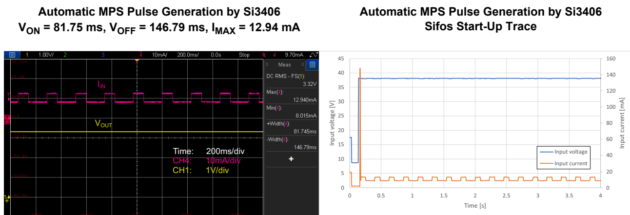
Figure 18. Si3406-ISO-FB EVB, 3.3 V, Class 2 PD Automatic Maintain Power Signature (MPS) Generation
