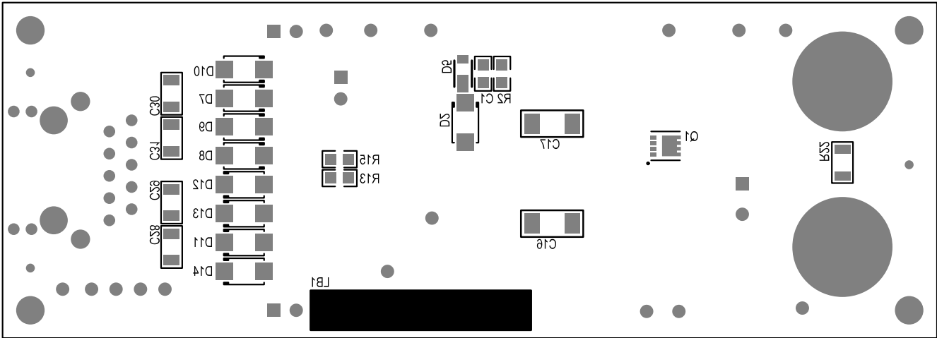
Figure 68. Bottom Silkscreen
