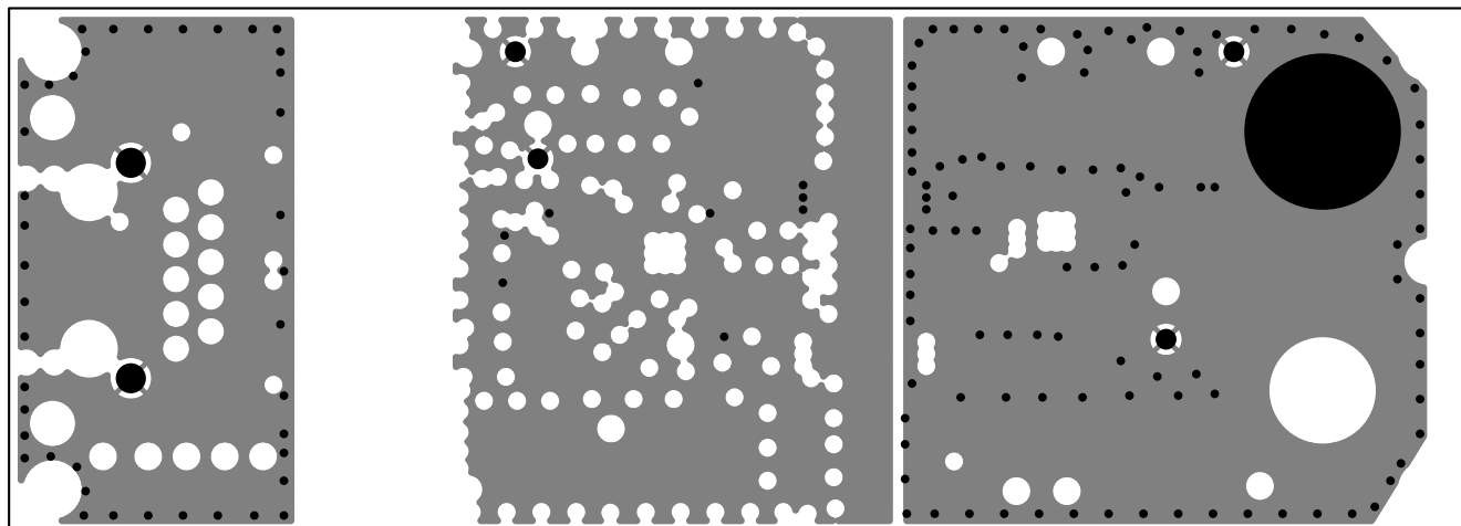
Figure 65. Internal 1 (Layer 2)
