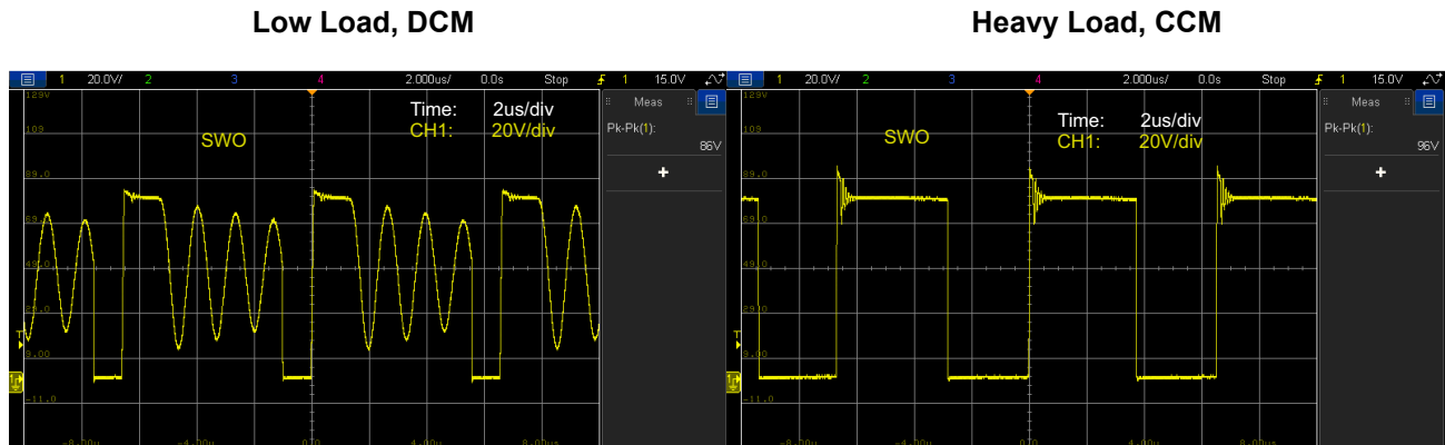
Figure 35. Si3406-ISO-FB EVB, 5 V, Class 2: SWO Waveform in Discontinuous Conduction Mode (DCM) at Low Load (Left), and in Continuous Conduction Mode (CCM) at Heavy Load (Right)
