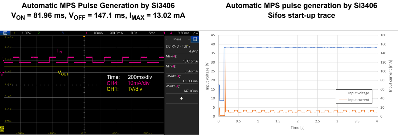
Figure 37. Si3406-ISO-FB EVB, 5 V, Class 2 PD Automatic Maintain Power Signature (MPS) Generation
