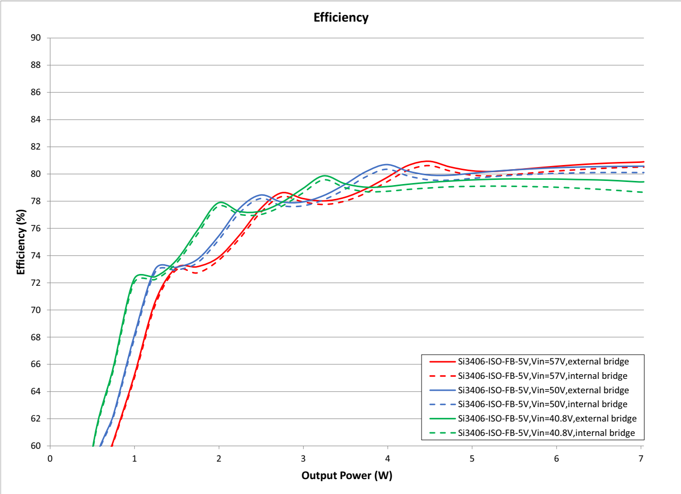
Figure 26. Si3406-ISO-FB End-to-End Efficiency Chart with Internal and External (S1B) Input Bridge Diodes: 40.8 V, 50 V and 57 V Input, 5 V Output, Class 2
