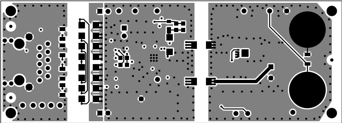
Figure 67. Bottom Layer
