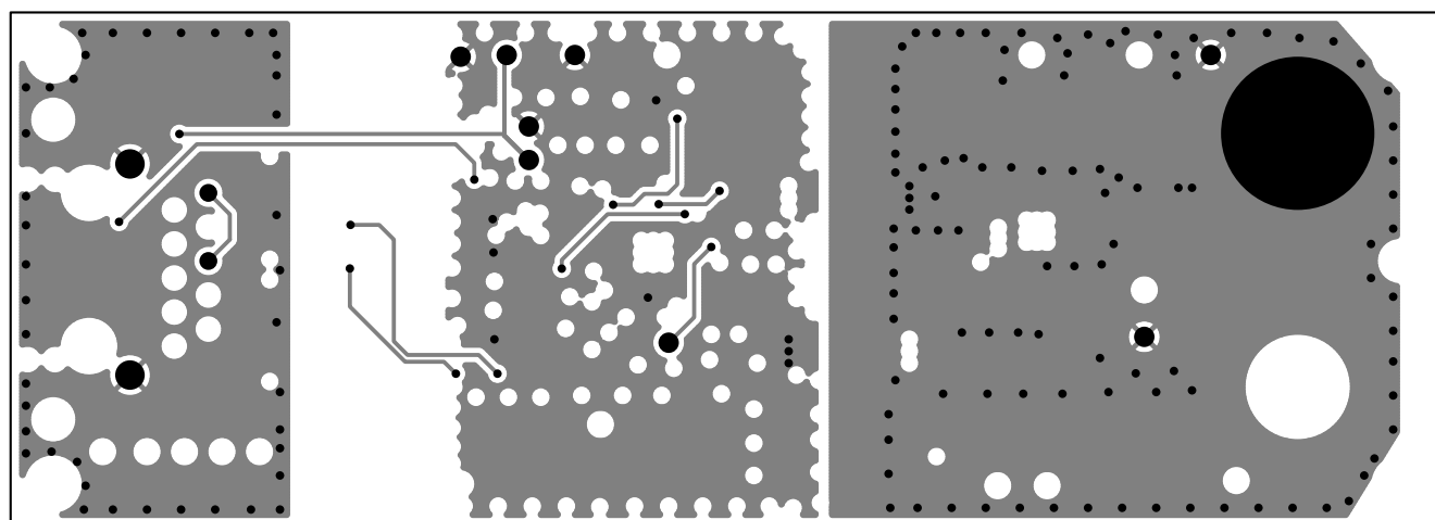
Figure 66. Internal 2 (Layer 3)
