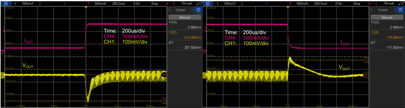
Figure 30. Si3406-ISO-FB EVB, 5 V, Class 2 PD Output Load Step Transient Test
