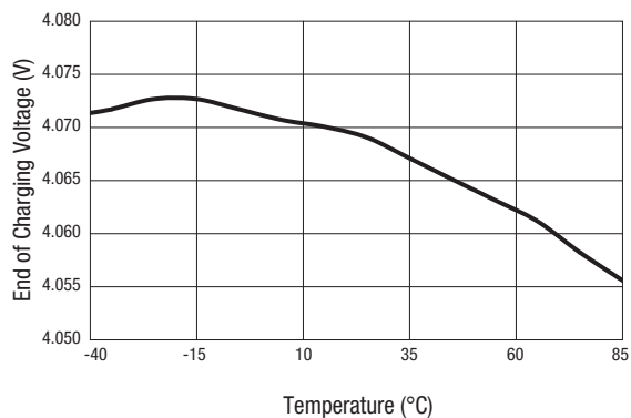
Figure 6. Recharging Voltage vs Temperature ( V_{IN} = 5\text{ V} )
