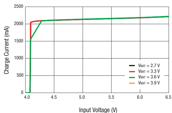
Figure 10. Charging Current vs Input Voltage ( T = 85\text{ }^{\circ}\text{C} )
