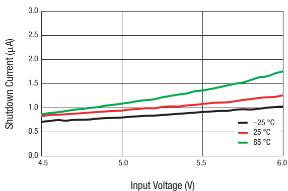
Figure 8. Shutdown Current vs Input Voltage
