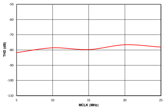
Figure 4.19. Si8935 Total Harmonic Distortion vs. MCLK (MHz)
