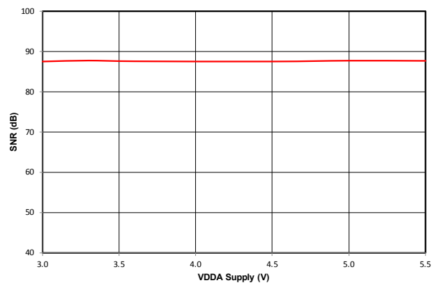
Figure 4.13. Si8935 Signal-to-Noise Ratio (dB) vs. VDDA Supply (V)
