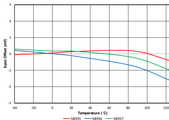
Figure 4.21. Input Offset (mV) vs. Temperature (°C)
