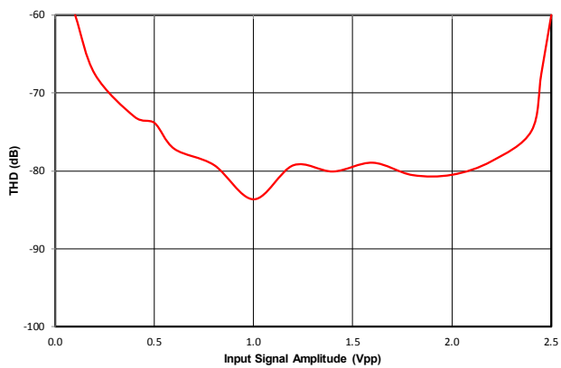
Figure 4.17. Si8935 Total Harmonic Distortion vs. Input Signal Amplitude (mV)
