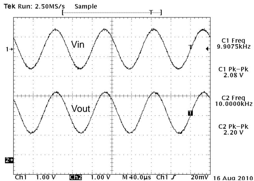
Figure 8. Circuit 1 Waveform ( V_{in} = 2 \text{ Vpp} , 10 kHz)
