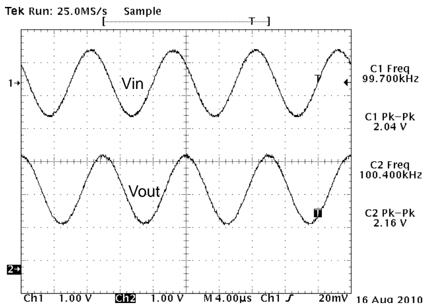
Figure 9. Circuit 1 Waveform ( V_{in} = 2 \text{ Vpp} , 100 kHz)
