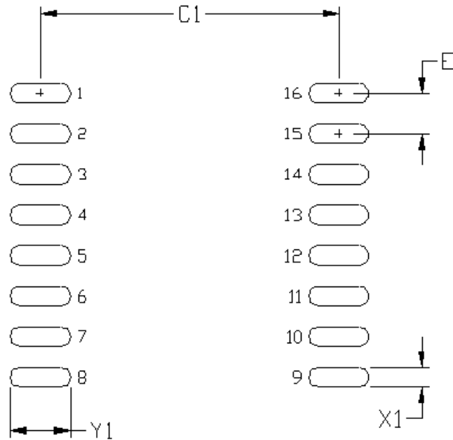
Figure 6.2. PCB Land Pattern: 16-Pin Wide Body SOIC
