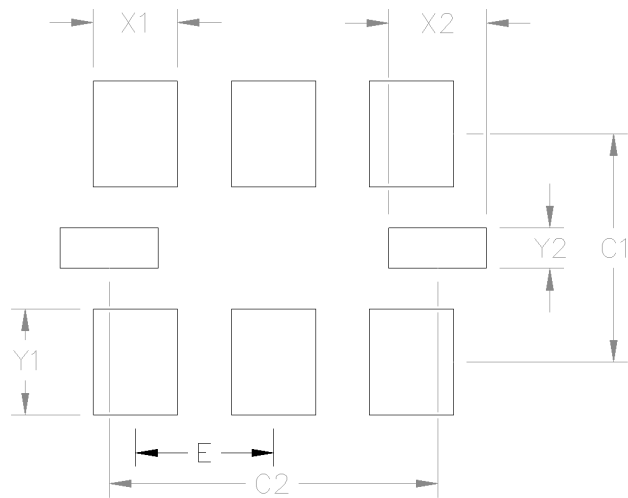
Figure 6.1. Si567 (5x7 mm) PCB Land Pattern
