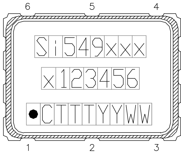
Figure 8.1. Mark Specification
