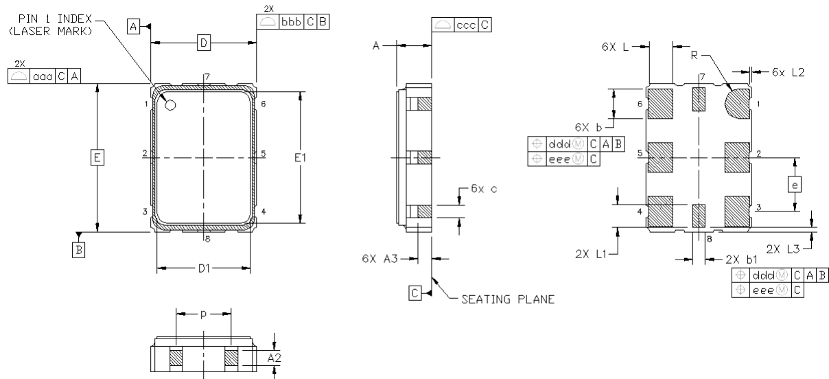
Figure 5.1. Si547 (5x7 mm) Outline Diagram
