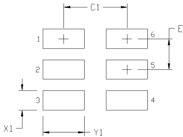
Figure 6.2. Si540 (3.2×5 mm) PCB Land Pattern
