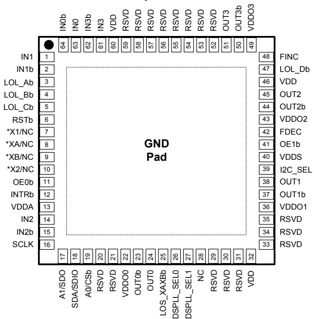
Si5396C/D/L/M (64-QFN and 64-LGA)
