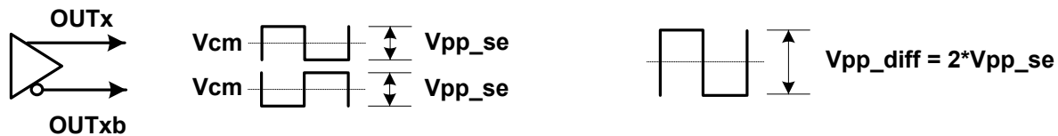
Differential Output Test Configuration
