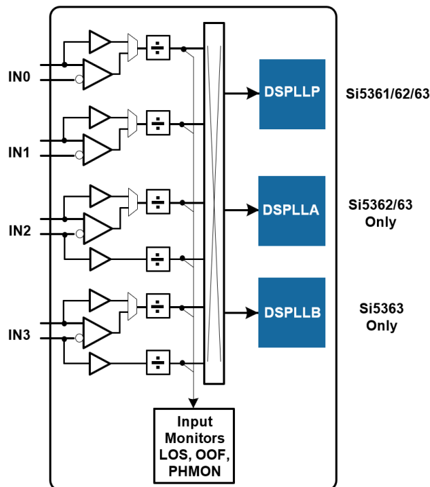
Figure 17. Input Structure
