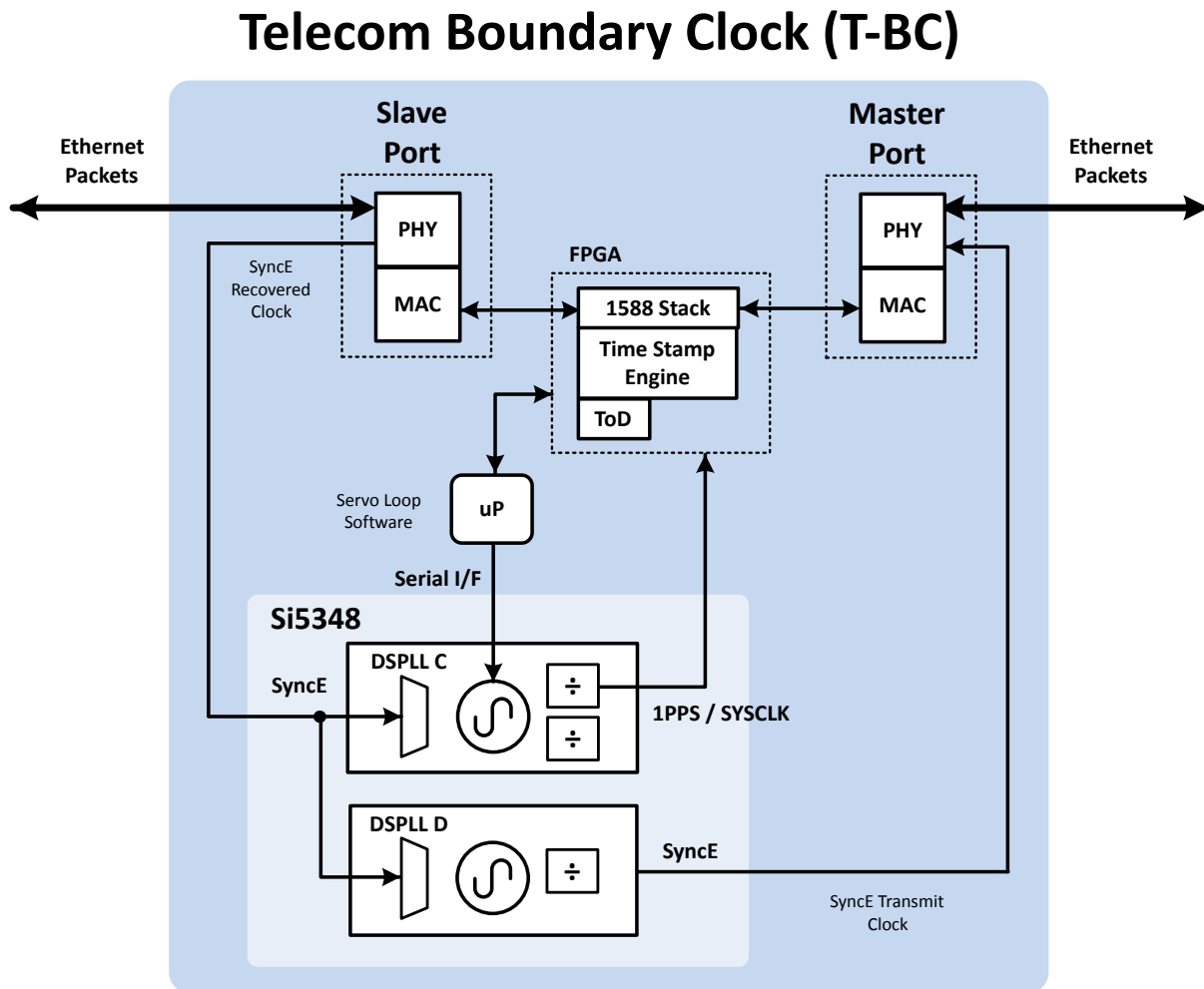
Figure 7.1. Using the Si5348 as a Telecom Boundary Clock
