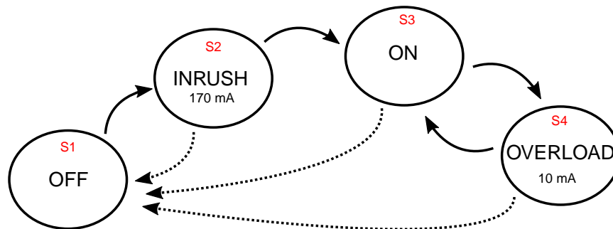
Figure 2.4. Hotswap Switch 4-State Machine
