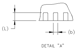
Figure 6.1. 20 引脚, QFN 封装
