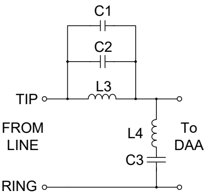
Figure 17. Billing-Tone Filter
