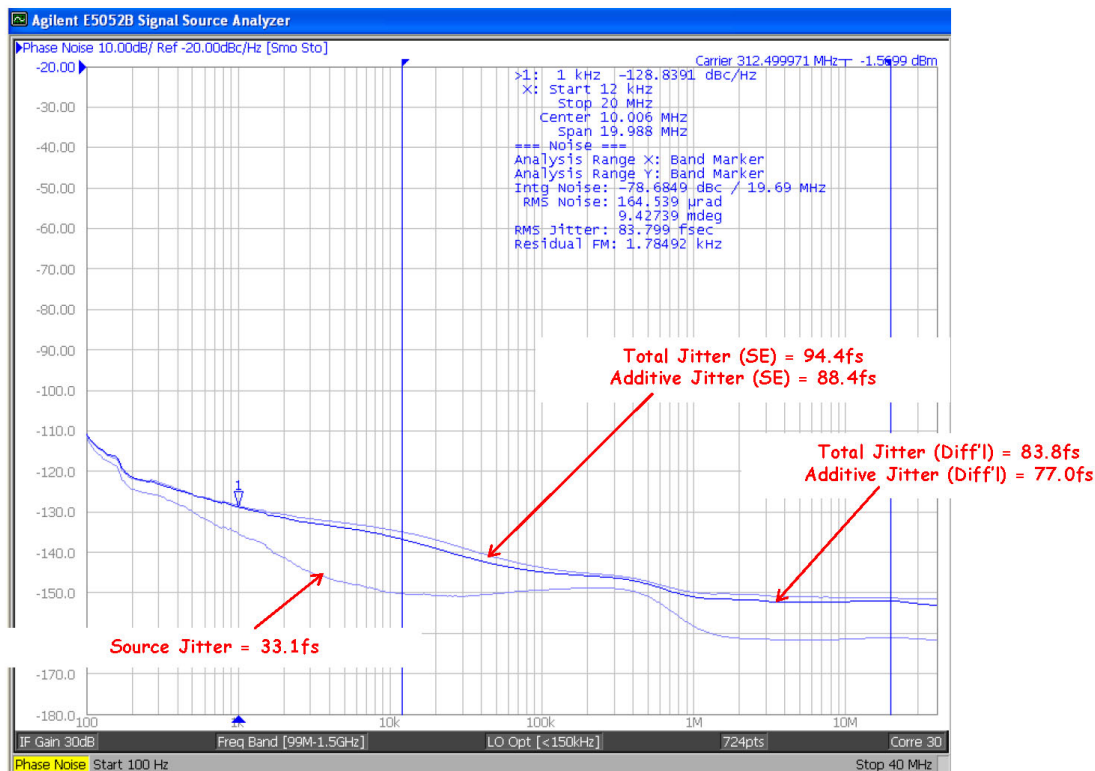
Figure 14. Single-ended Total Jitter (312.5 MHz)
