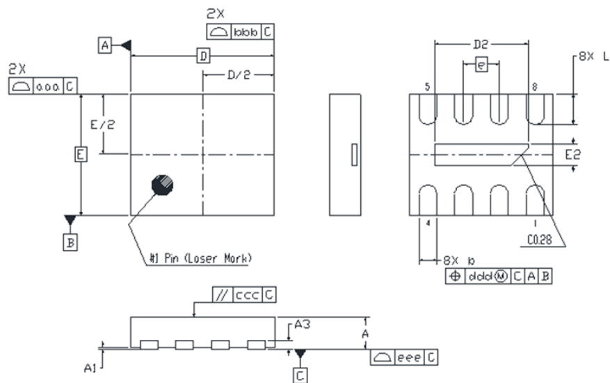
Figure 7.1. 8-pin TDFN
