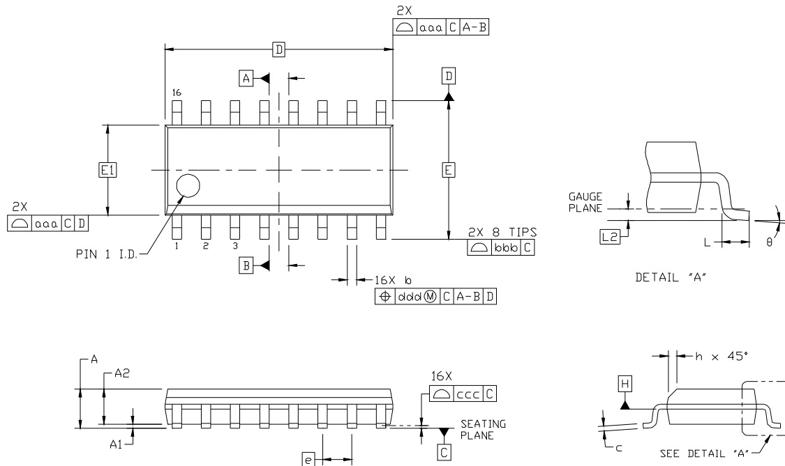
Figure 3. 16-Pin SOIC
