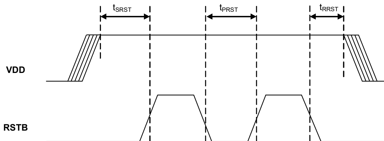
Figure 1. Reset Timing
