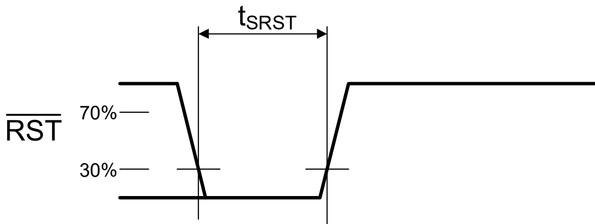
Figure 1. Reset Timing
