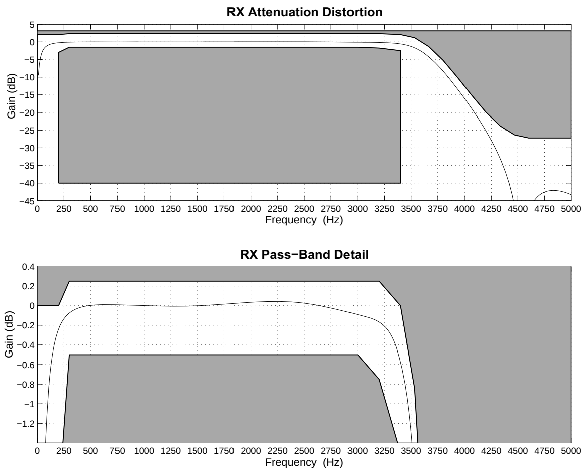
Figure 5. Receive Path Frequency Response
