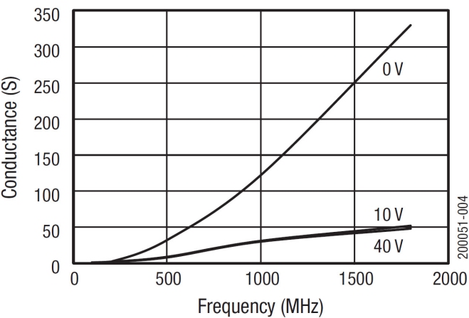
Figure 4. Conductance vs Frequency and Reverse Voltage
