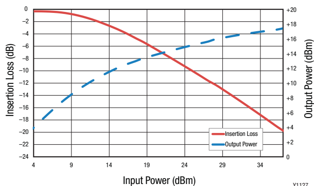
Figure 4. Insertion Loss and Output Power vs Input Power ( f = 1.0\text{ GHz} , Board Loss Included)
