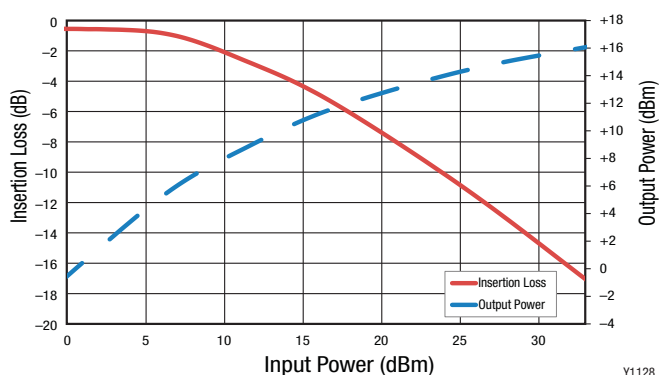
Figure 5. Insertion Loss and Output Power vs Input Power ( f = 2.5\text{ GHz} , Board Loss Included)
