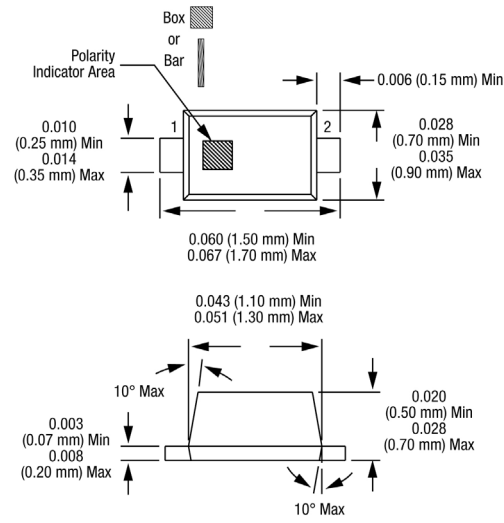
Dimensions are in inches (millimeters shown in parentheses) 200048-006
