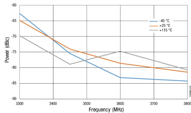
Figure 16. 3rd Harmonic vs Frequency Across Temperature (P OUT = +28 dBm, CW)
