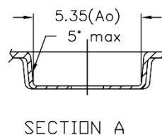
Figure 24. SKY66318-11 Tape and Reel Dimensions
