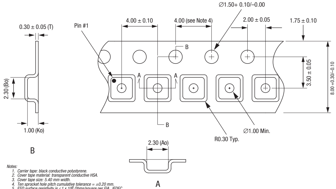
Figure 11. CLA4606-085LF Tape and Reel Dimensions
