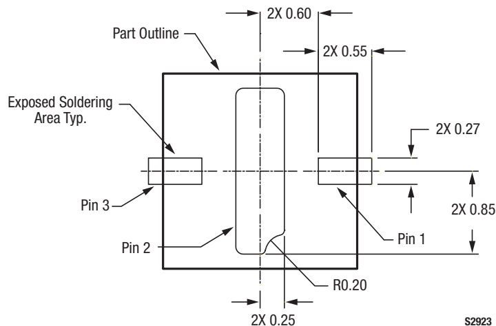
Figure 8. CLA4606-085LF PCB Layout Footprint
