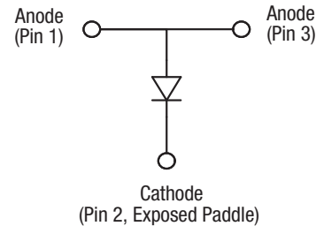
Figure 1. CLA4610-085LF Block Diagram
