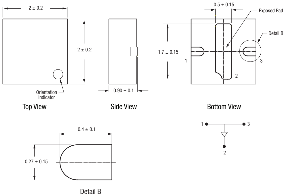
Figure 10. SMP1330-085LF Package Dimensions
