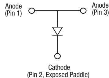
Figure 1. SMP1330-085LF Block Diagram
