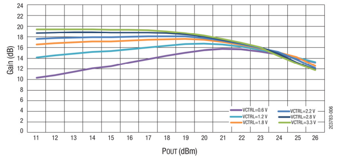
Figure 6. Gain vs POUT vs VCTRL (VCC1 = VCC2 = 1.8 V), f = 2440 MHz, CW
