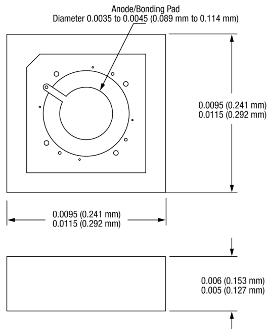
Figure 8. 571-011 Package Dimensions
