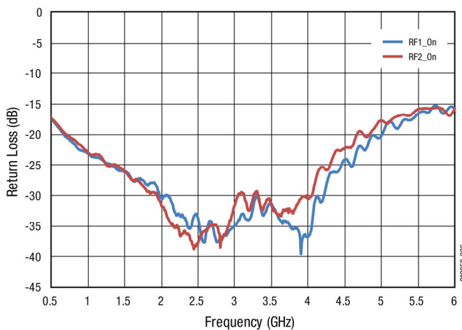
Figure 6. Typical Return Loss
