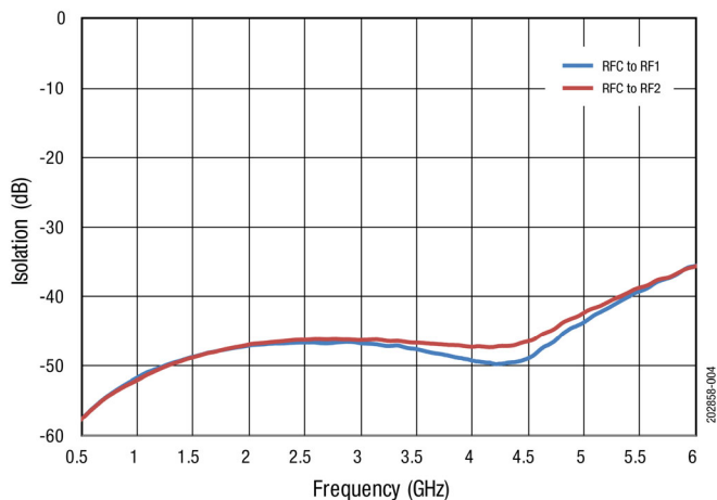
Figure 4. Typical Isolation
