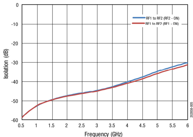
Figure 5. Typical Isolation
