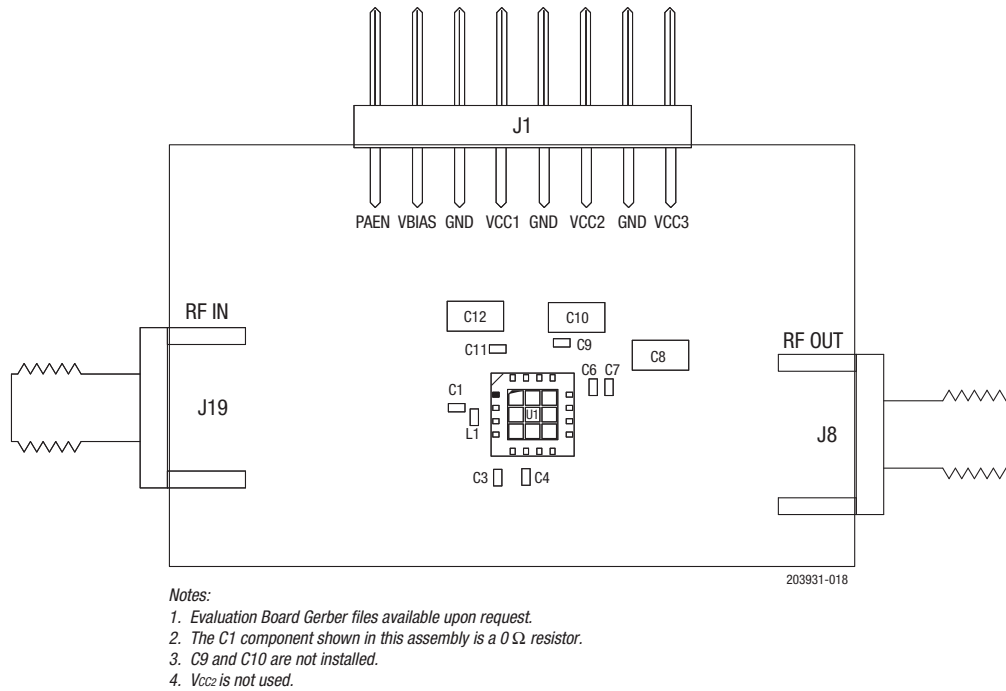
Figure 18. Evaluation Board Assembly Drawing
