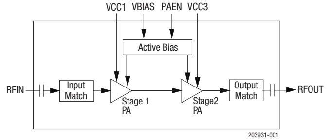
Figure 1. SKY66296-11 Block Diagram
