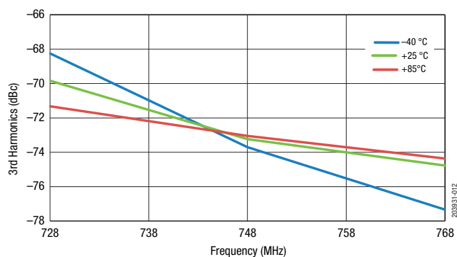
Figure 12. 3 rd Harmonic vs Frequency Across Temperature @ Pout = +28 dBm (CW)
