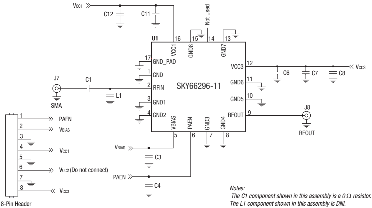
Figure 17. SKY66296-11 Application Schematic
