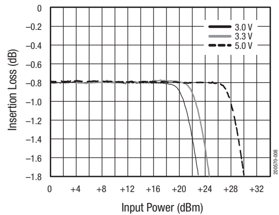
Figure 8. Insertion Loss vs Input Power Over Voltage
