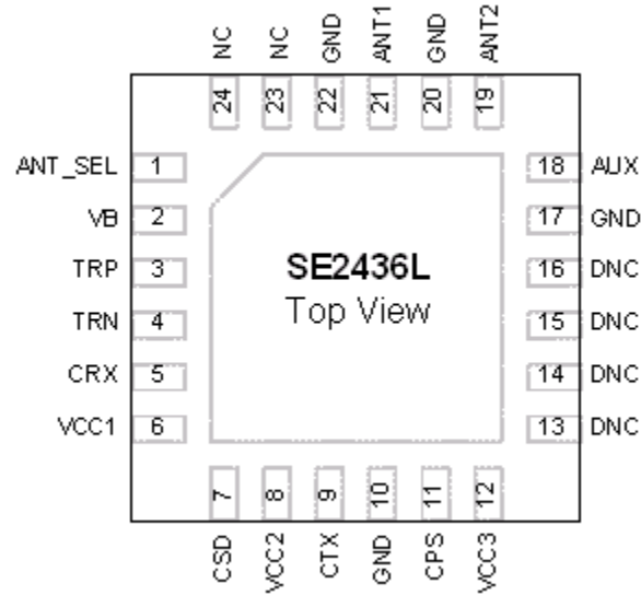
Figure 2: SE2436L Pinout
