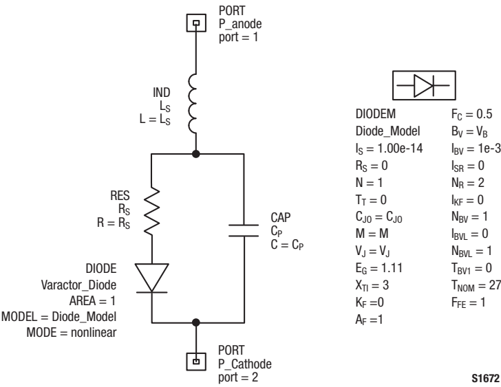
Figure 3. SPICE Model
