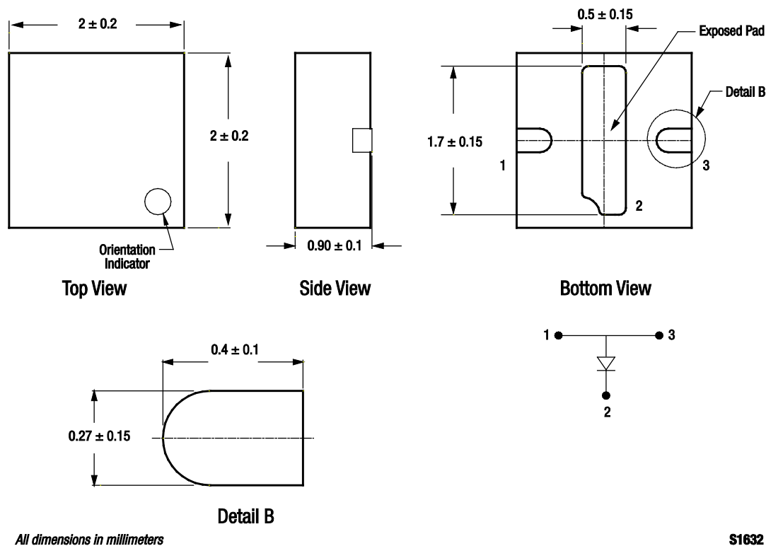
Figure 10. SMP1302-085LF QFN Package Dimension Drawing
