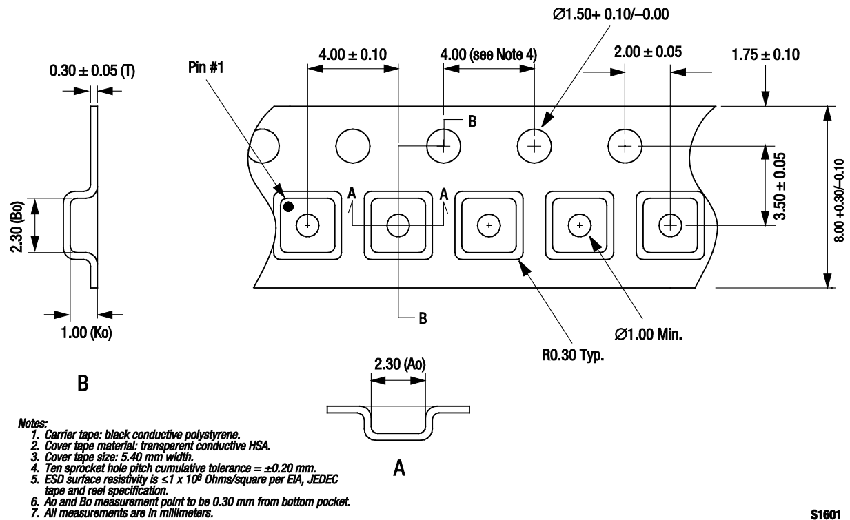
Figure 11. SMP1304-085LF Tape and Reel Dimensions
