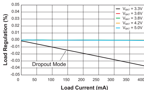
Main SD Load Regulation vs. Output Current (V PVM = V BAT ; V MSD = 3.3V; L = 3.3μH; C OUT = 4.7μF)
