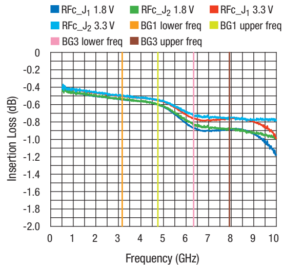
Typical Insertion Loss
