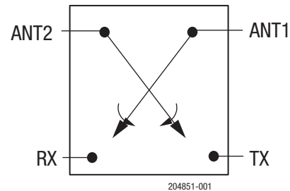
Figure 1. SKYA21070 Block Diagram
