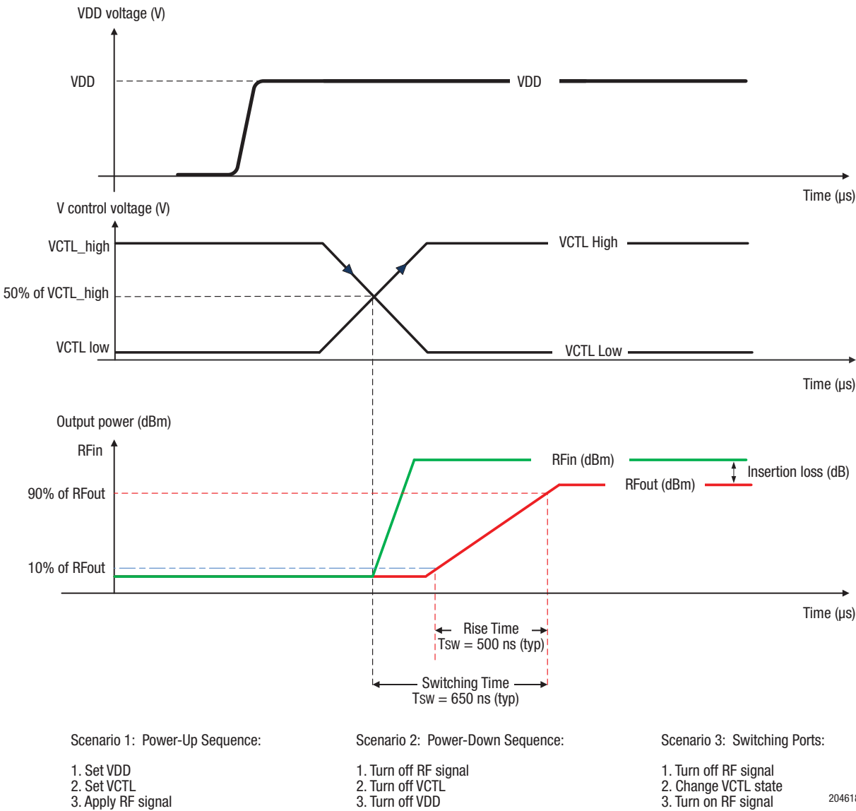
Figure 3. SKYA21024 Timing Diagram
