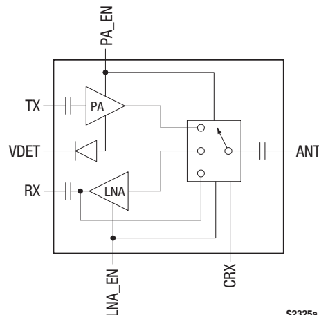
Figure 1. SKY85711-21 Block Diagram
