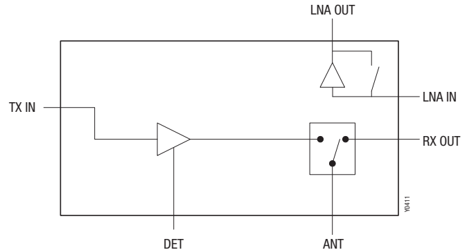
Figure 1. SKY85710-11 Block Diagram
