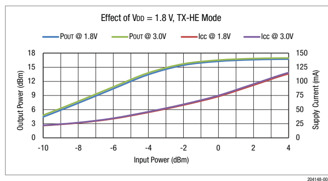
Figure 5. Effect of Lowering V_{DD} ( V_{CC1} = V_{CC2} = 1.8\text{ V} , TX-HE mode, f = 2440\text{ MHz} )
