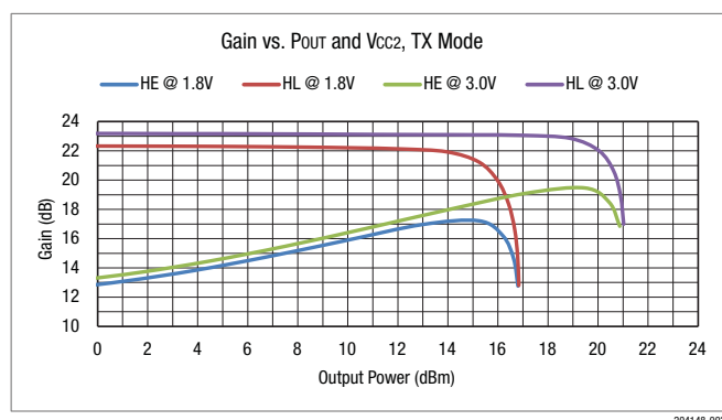
Figure 3. Effect of CHL on Gain ( V_{CC1} = 1.8\text{ V} , V_{DD} = 3.0\text{ V} , f = 2440\text{ MHz} )
