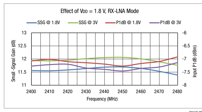
Figure 6. Effect of Lowering V_{DD} ( V_{CC1} = V_{CC2} = 1.8\text{ V} , P_{IN} = -25\text{ dBm} , RX-LNA Mode)
