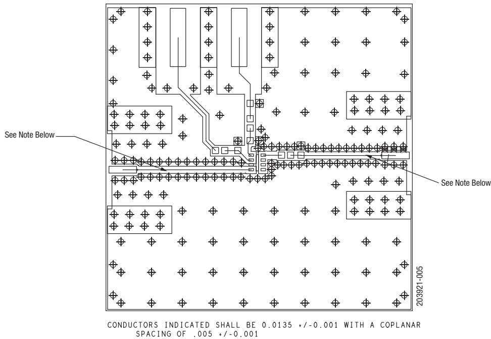
Figure 5. SKY65723-11 Evaluation Board Layer Details
