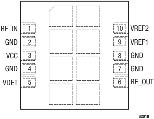
Figure 2. SKY65174-21 Pinout (Top View)
