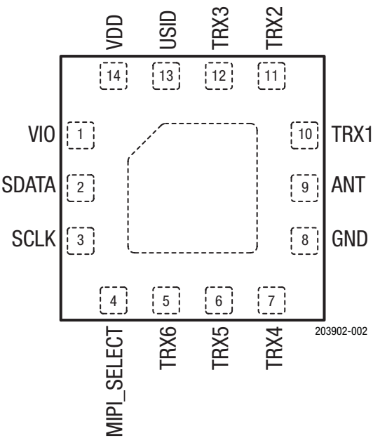
Figure 2. SKY13525-646LF Pinout (Top View)
