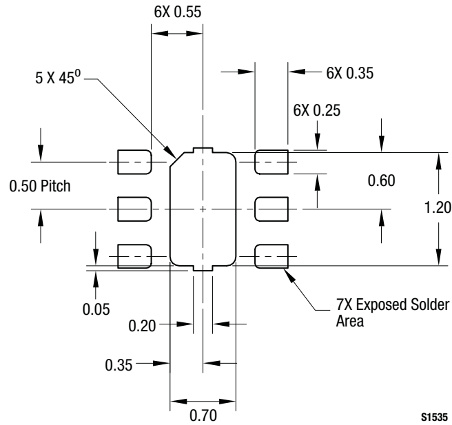
Figure 11. SKY13411-374LF PCB Layout Footprint (Top View)
