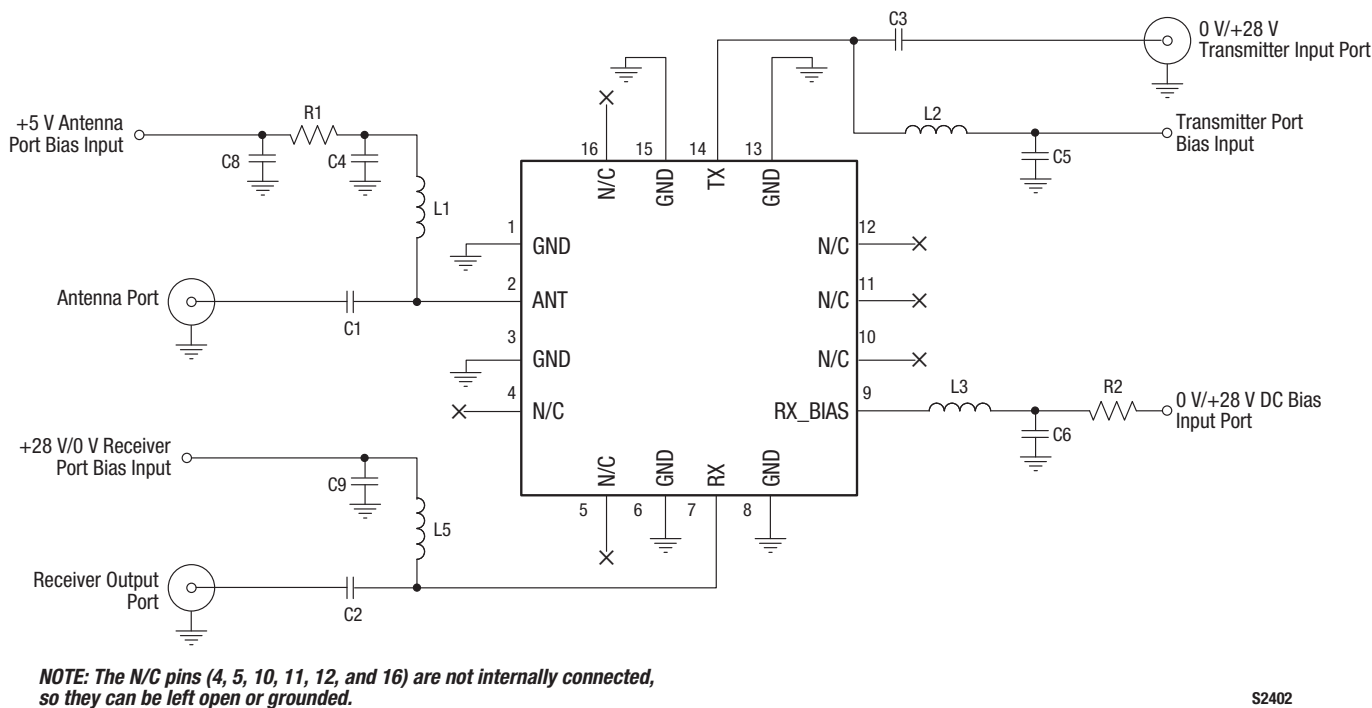
Figure 12. Evaluation Board Schematic
