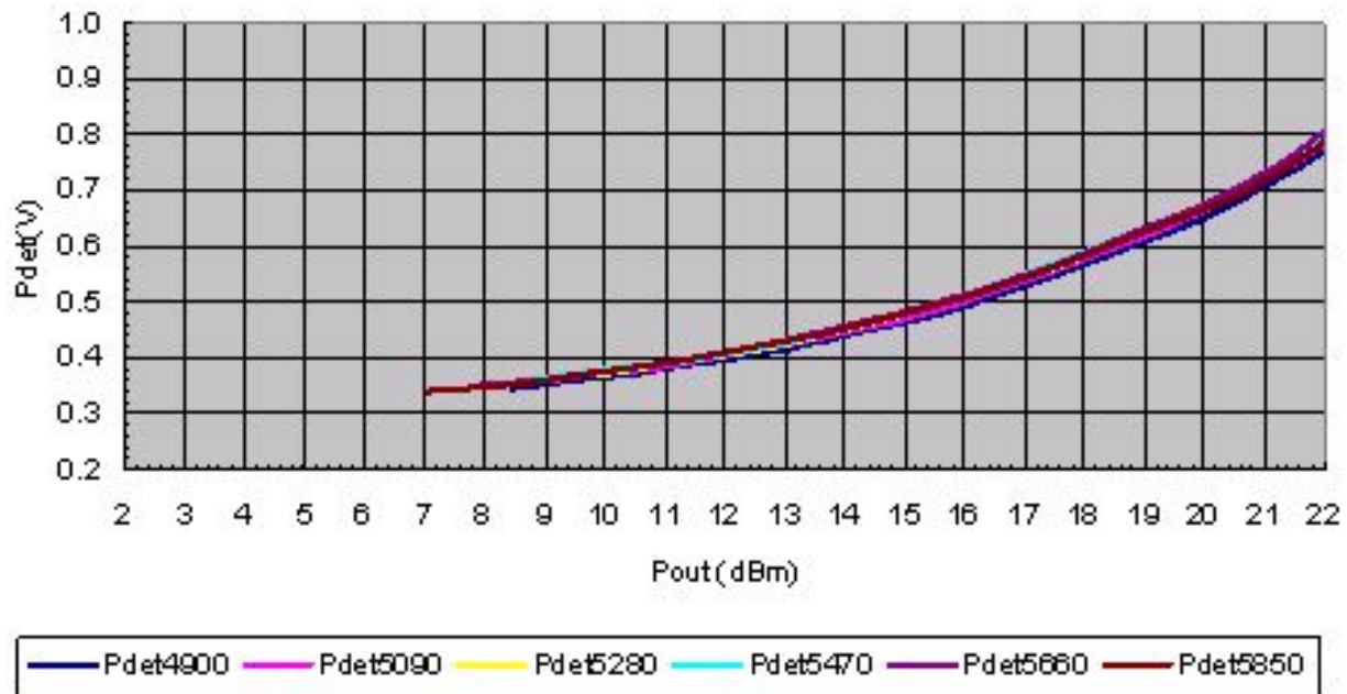
Figure 3: SE5007T Power Detector Characteristic
